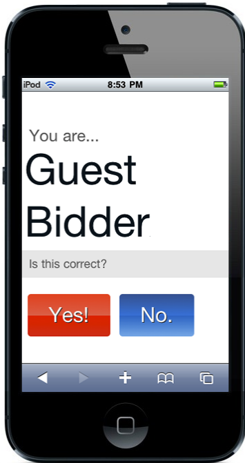
Welcome Screen
